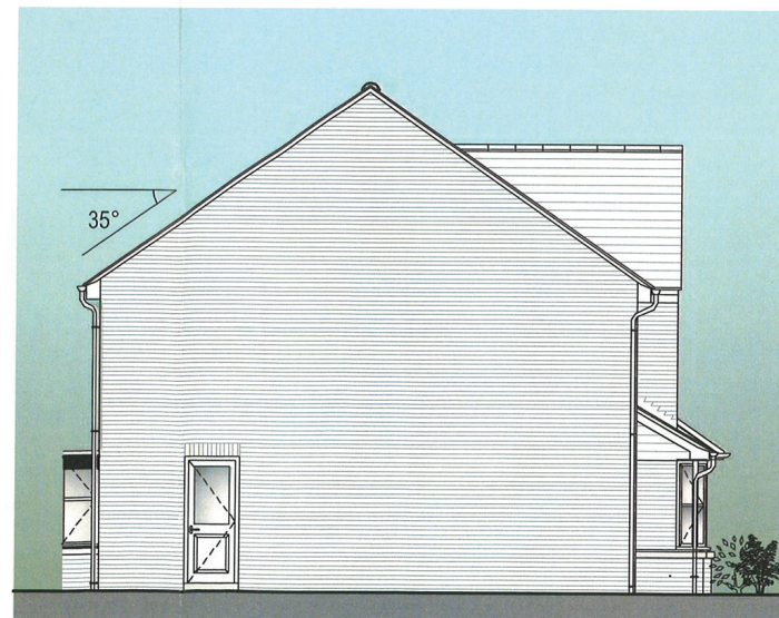
LEFT GABLE ELEVATION
